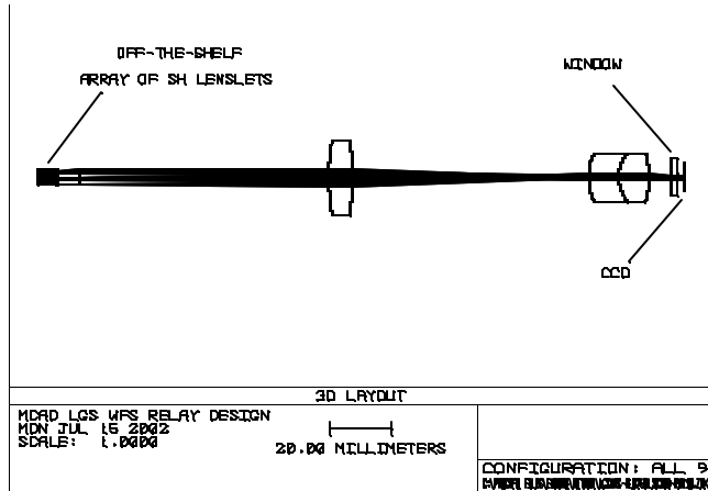
Figure 10: LGS WFS SH spot relay.
